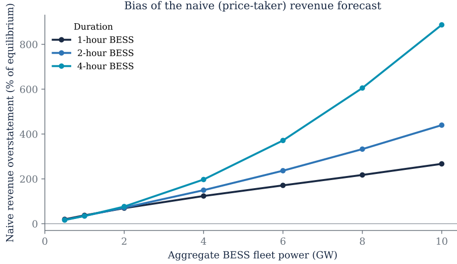
Figure 3: Bias of the naive (price-taker) revenue forecast as a function of fleet size, by storage duration. Positive bias means the naive forecast overstates revenue. Bias is monotone in fleet size, and monotone in duration for fleets of 2 GW and above (below 2 GW the ordering reverses). For two-hour batteries the naive overstatement is 150% at a 4 GW effective price-setting fleet, 236% at 6 GW, and 333% at 8 GW; the 4–8 GW band is the one in which the widely quoted “100–300%+” figures arise. As discussed in the text, this aggregate single-zone capacity is not the \sim 25 GW system-wide GB installed base projected for 2030.
