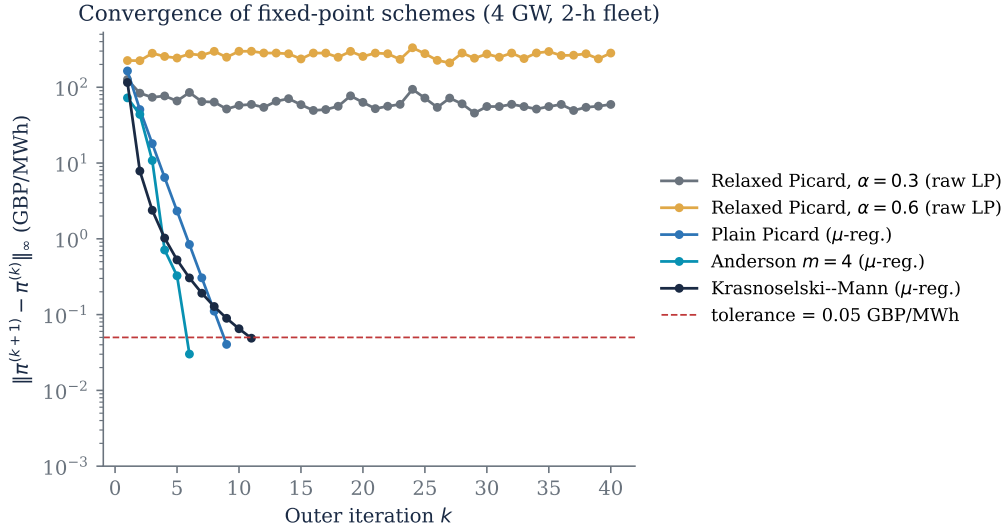
Figure 6: Convergence of five fixed-point iteration schemes on the same 4 GW, 2-hour problem (4-week certificate window; regularised schemes use the certificate \mu , chosen above the realised supply-curve slope). Relaxed Picard on the raw dispatch operator fails at the 0.05 GBP/MWh tolerance under both dampings: \alpha = 0.6 oscillates, \alpha = 0.3 stagnates in the tens of GBP/MWh. On the regularised map every scheme converges — Anderson (depth m = 4 ) in 6 iterations, plain Picard in 9, KM in 11: regularisation, not averaging, is what makes the iteration converge. KM is the production scheme for the guarantee that survives at the non-expansive boundary; its advantage over raw Picard is consistent across all fleet sizes considered.
